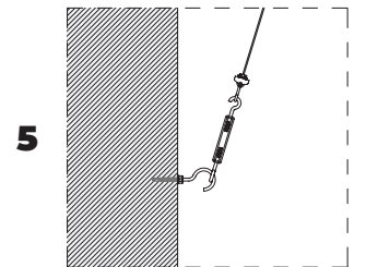
FIXING STEEL ACCESSO- RIES DETAIL
