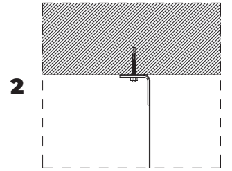
CONCRETE STEEL ANCHOR DETAIL
