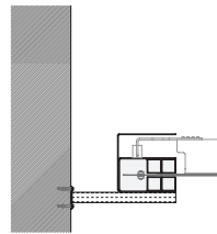
SECTION HORIZONTAL
